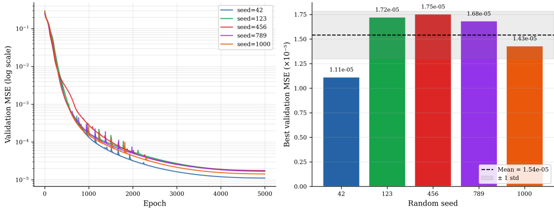
Figure 10: Training seed robustness across five random initialisations. Left: validation MSE curves; right: best validation MSE per seed.
